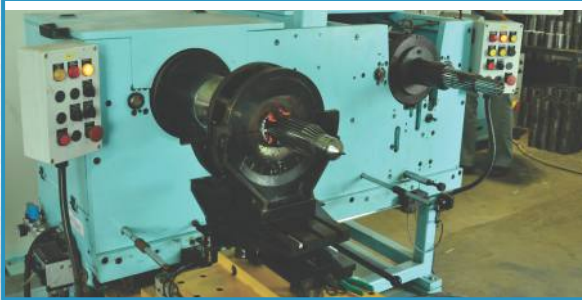
Automatic Winding
